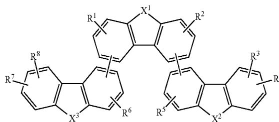
[Chemical Formula 3]
