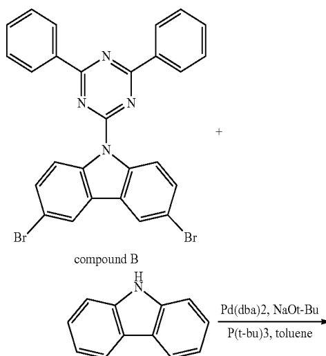
[Reaction Scheme 2]
