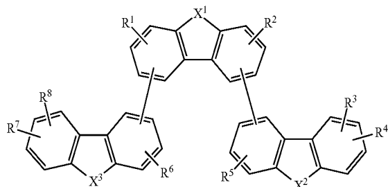
[Chemical Formula 3]
