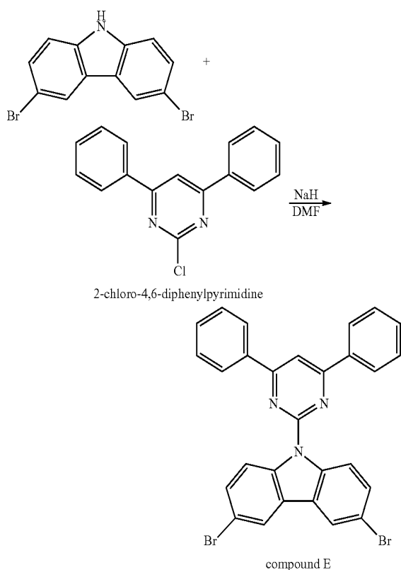
[Reaction Scheme 4]
