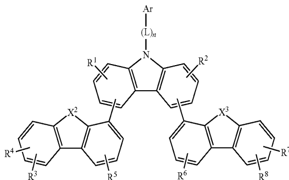
[Chemical Formula 4]
