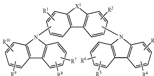
[Chemical Formula 1]
