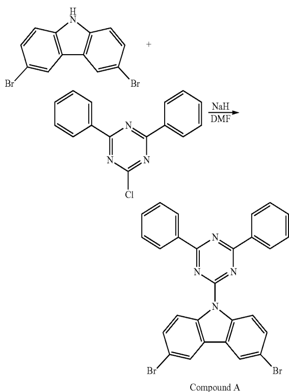
[Reaction Scheme 1]
